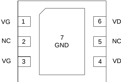
Figure 3. CAQ4030L Pinout
