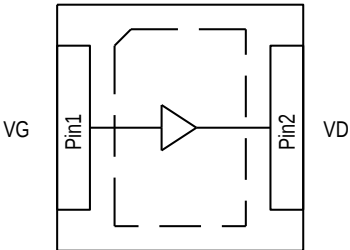
Figure 2. CAQ4030L Function Block Diagram
